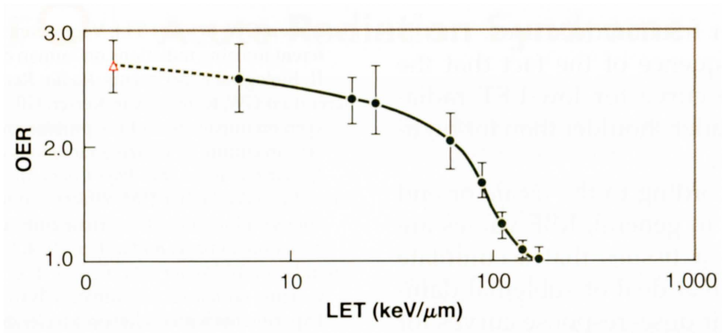
OER as a function of LET. Measurements of OER were made with cultured cells of human origin. Closed circles refer to monoenergetic charged particles, the open triangle to 250-kVp x-rays with an assumed track average LET of 1.3 keV/μ. (From Barendsen GW, Koot CJ, van Kersen GR, Bewley DK, Field SB, Parnell CJ: Int J Radiat Biol 10:317–327, 1966)
