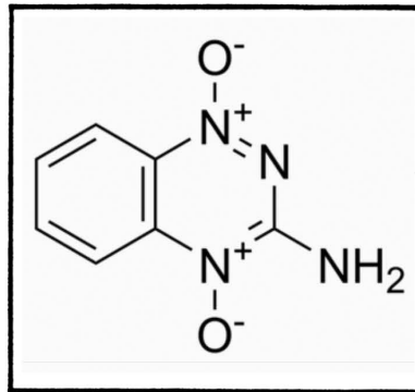
3-amino-1,2,4-benzotriazine 1,4-dioxide
