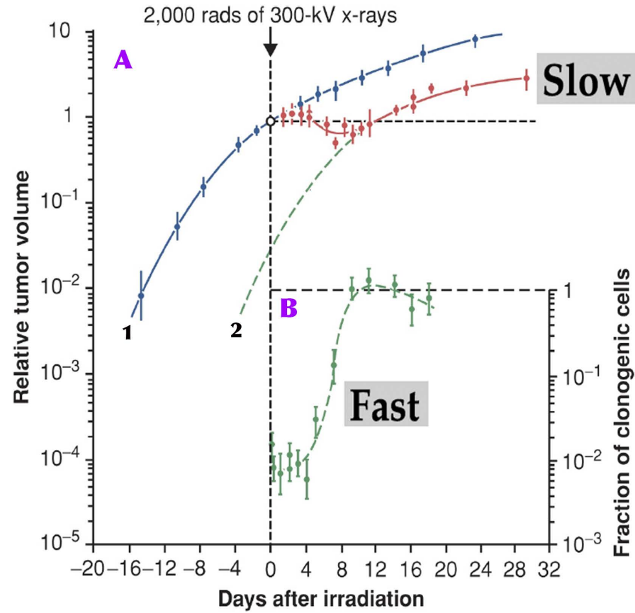
Accelerated repopulation. Growth curves of a rat rhabdomyosarcoma showing the shrinkage, growth delay, and subsequent recurrence following treatment with a single dose of 20 Gy (2,000 rad) of x-rays. A: Curve 1: Growth curve of unirradiated control tumors. Curve 2: Growth curve of tumors irradiated at time t = 0 , showing tumor shrinkage and recurrence. B: Variation of the fraction of clonogenic cells as a function of time after irradiation, obtained by removing cells from the tumor and assaying for colony formation in vitro. (From Hermens AF, Barendsen GW: Eur J Cancer 5:173-189, 1969)
